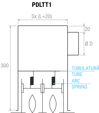
Fixare plenum cu arcuri CM Fixing the plenum by springs CM
