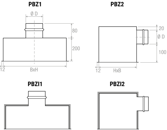
Plenum izolat la exterior, grosime 6 mm Plenum externally insulated thickness 6 mm
