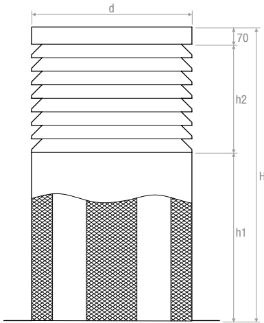
Versiune cu atenuator de zgomot Version with sound attenuator
