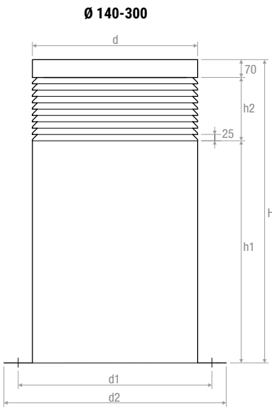
Versiune cu atenuator de zgomot Version with sound attenuator
