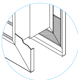
DETALIU INSERARE CONTRA-CADRU PARTICULAR INSERTION COUNTERFRAME
