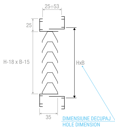
DETALIU INSERARE CONTRA-CADRU PARTICULAR INSERTION COUNTERFRAME
