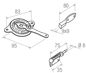
CM60
