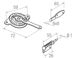
CM50
