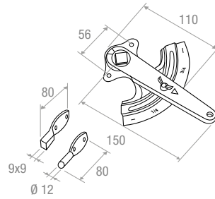
CM70
