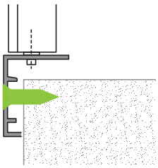
Fixation à vis Fixing with screws
