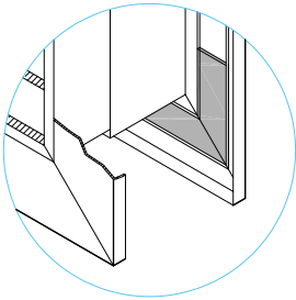
DETALLE INSERCIÓN CONTRAMARCO PARTICULAR INSERTION COUNTERFRAME
