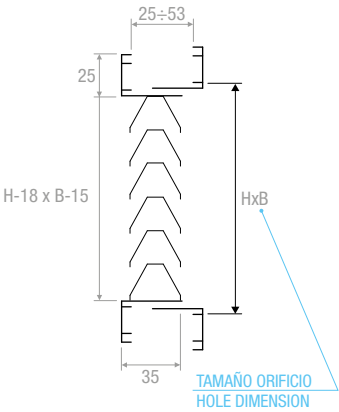
DETALLE INSERCIÓN CONTRAMARCO PARTICULAR INSERTION COUNTERFRAME
