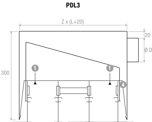
Fissaggio al plenum con staffe inclinate CVL cavalletti Fixing to the plenum by inner mounting bridge inclined CVL
