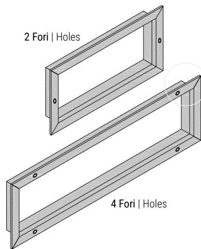
1 Ø 3,5 Foro svasato | Countersunk hole
