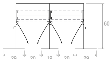
DLF250 2 Schlitz - Slots
