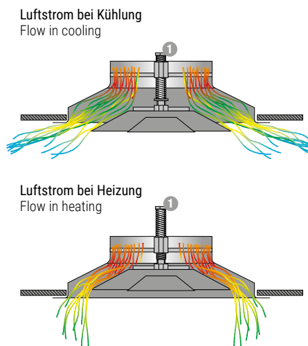
1 Thermostatelement | Thermostatic actuator
