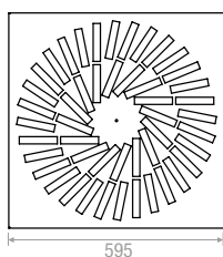
48 Schlitz | Slots
