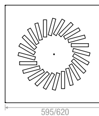
24 Schlitz | Slots
