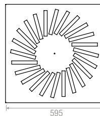
24 Schlitz | Slots
