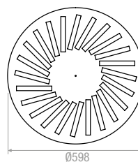
24 Schlitz | Slots
