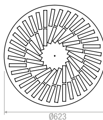
54 Schlitz | Slots
