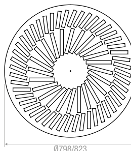
72 Schlitz | Slots
