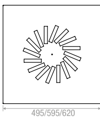
16 Schlitz | Slots
